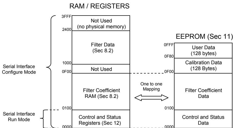
Figure 2. Memory Map
